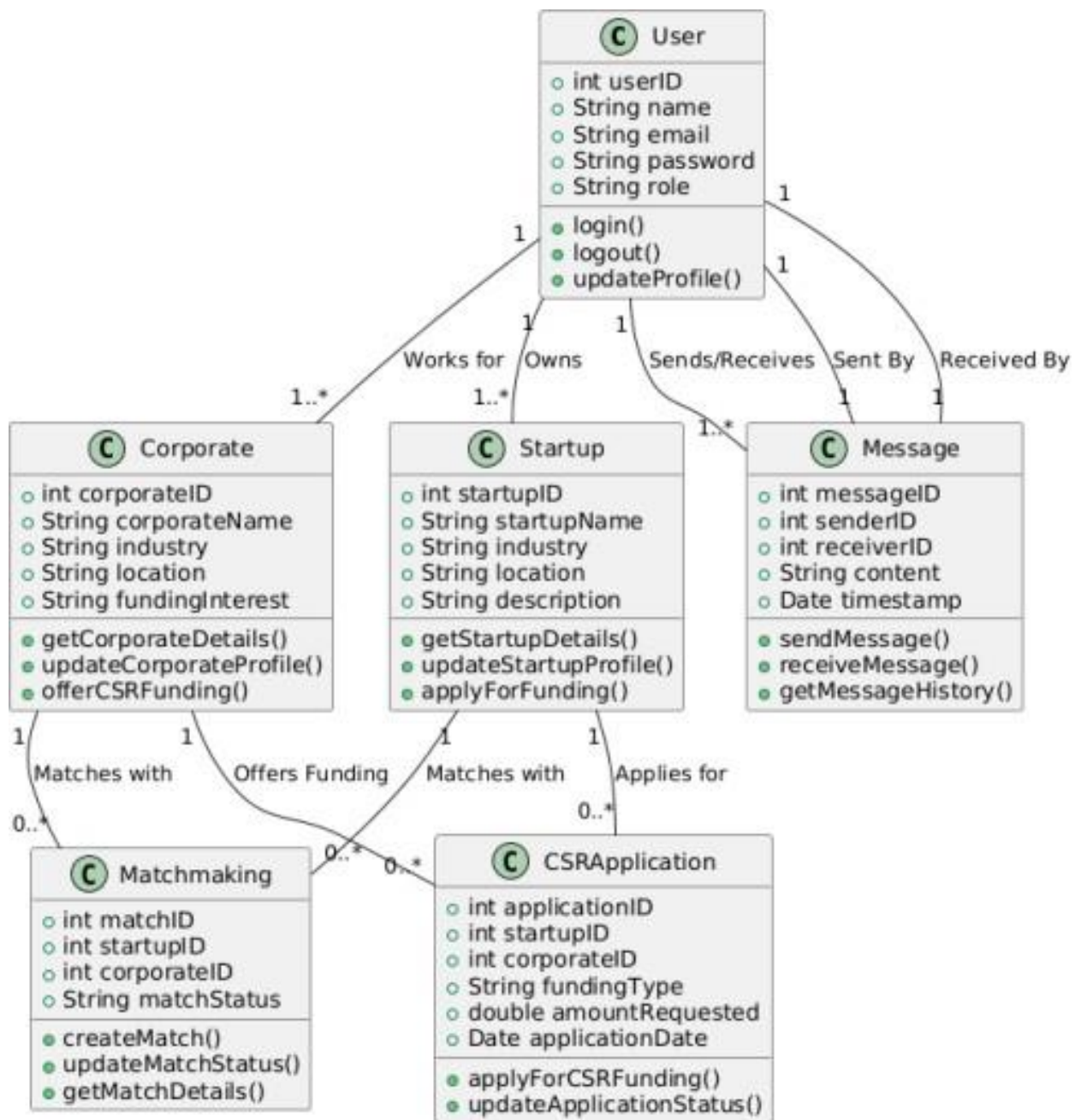
Figure 3.6: Class Diagram
