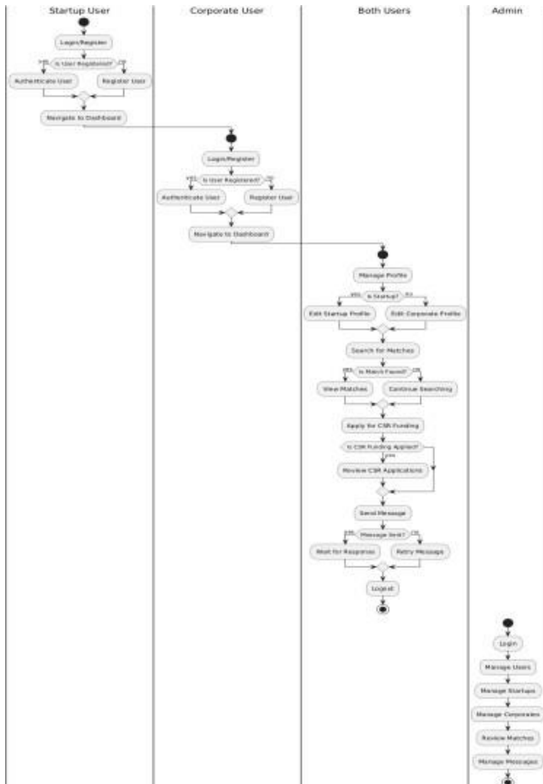
Figure 3.2: Activity Diagram:
